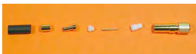
Components of the 245-CON-MIC connector. All connectors come with an assembly manual
