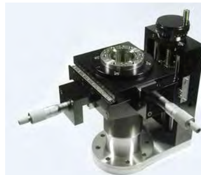
621-CMX-50-C40 with 63CF base flange option
